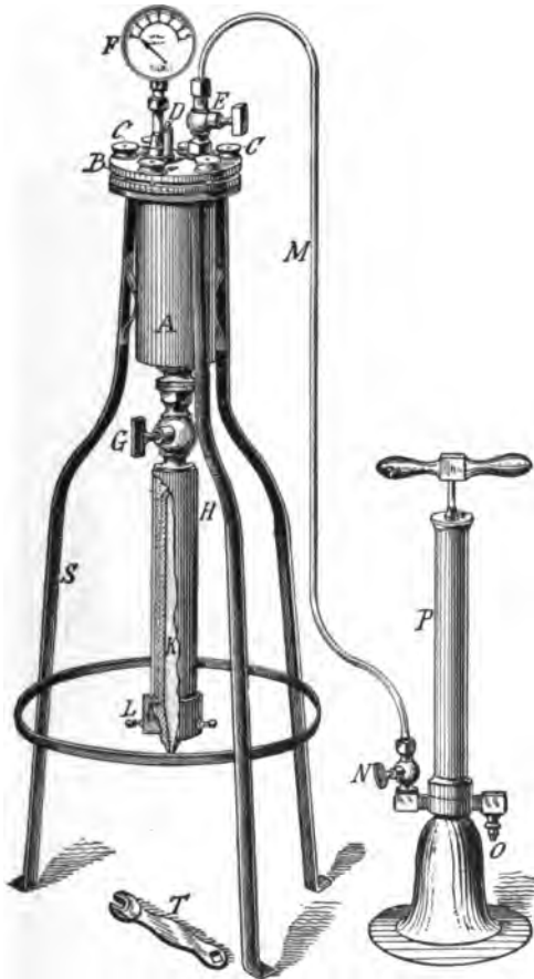
Fig. 41.—Pasteur-Chamberland filter arranged to filter under pressure.
